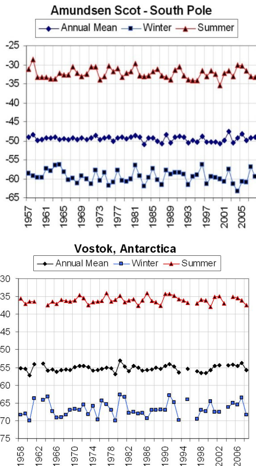
Figure 5.8.3.3.1. Temperature measurements at the South Pole (above) and Vostok (below). Note the lack of any indication of recent warming. Adapted from Easterbrook, D.J. (Ed.) 2011. Evidence-based climate science: Data opposing CO 2 emissions as the primary source of global warming . Elsevier.
