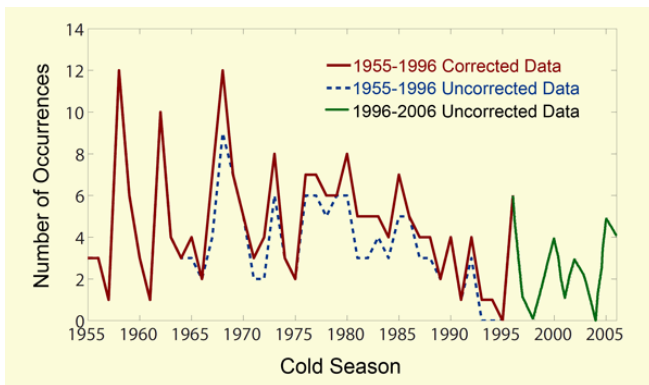
Figure 7.7.1.3.1.1. Cold-season occurrences of major precipitation events at Iqaluit, Nunavut, Canada. Adapted from Gascon, G., Stewart, R.E., and Henson, W. 2010. Major cold-season precipitation events at Iqaluit, Nunavut. Arctic 63 : 327–337.
