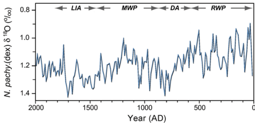
Figure 4.2.4.8.2.7. Proxy temperature reconstruction of N. pachyderma (dex) \delta^{18}\text{O} vs. time. Adapted from Sejrur, H.P., Hafliðason, H., and Andrews, J.T. 2011. A Holocene North Atlantic SST record and regional climate variability. Quaternary Science Reviews 30 : 3181–3195.
