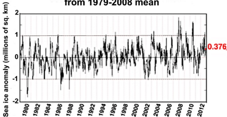
Southern Hemisphere sea ice anomaly from 1979-2008 mean
